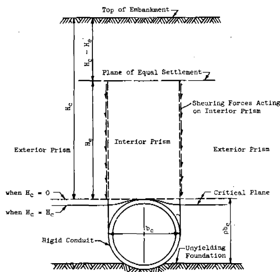
Fig. 1-2 Basic case for considering the action of an embankment over a positive projecting conduit
