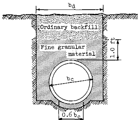
Type B—first class bedding
