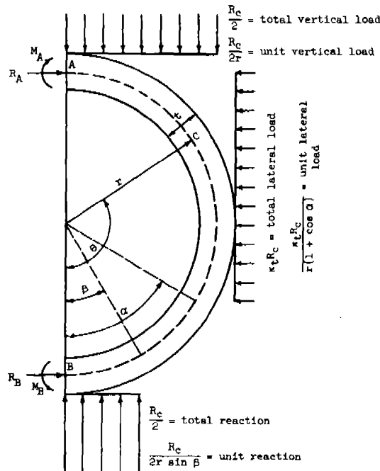
Fig. B-5 Assumed loads for actual field conditions
