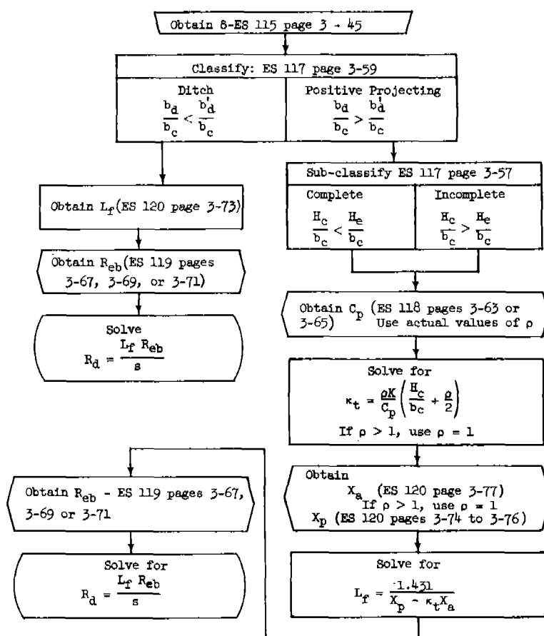
Fig. 2-3. Procedure for determining the safe supporting strength of a conduit installed as a ditch conduit or a positive projecting conduit.
