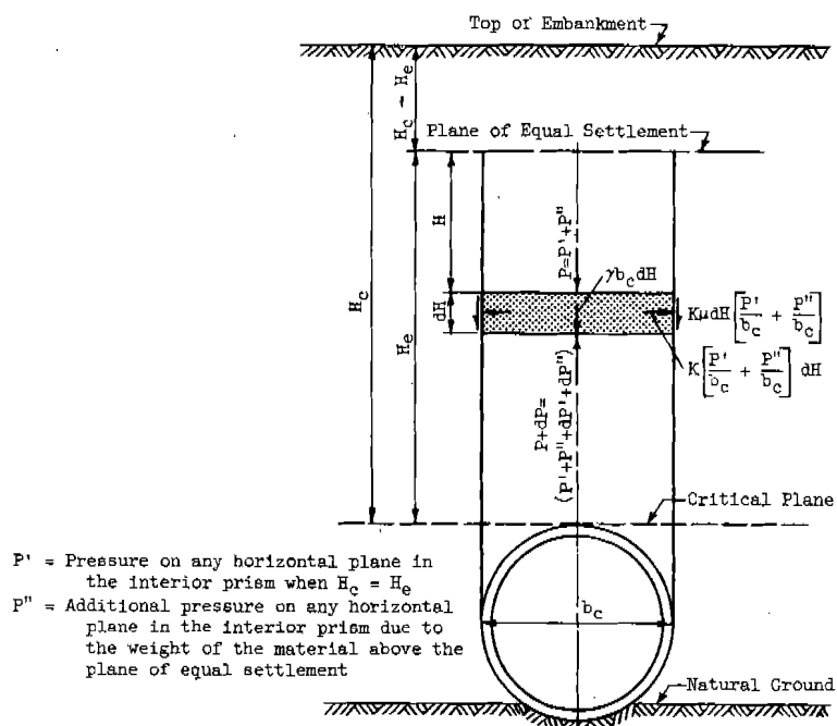
Fig. A-3 Forces used to determine the additional consolidation of the material in the interior prism
