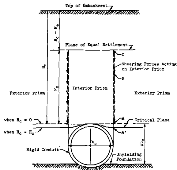
Fig. A-2 Basic case for considering the action of an embankment over a positive projecting conduit.
