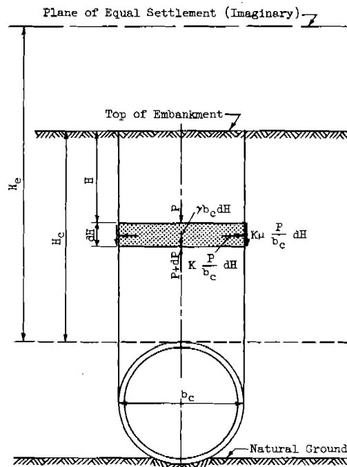
Fig. A-4 Loads on a horizontal element in the interior prism for the complete condition
