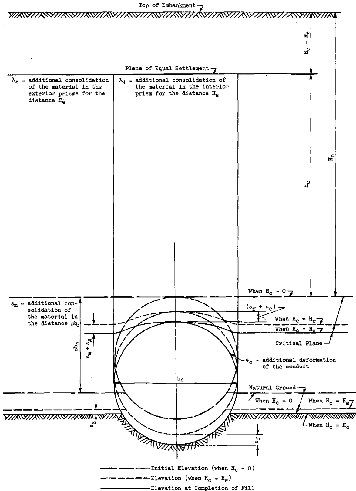
Fig. 1-3 Settlements which influence loads on positive projecting conduits
