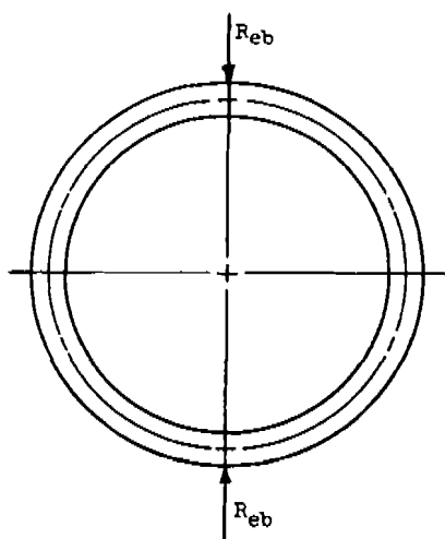
Fig. B-1a Assumed load distribution for the case of three-edge bearing
