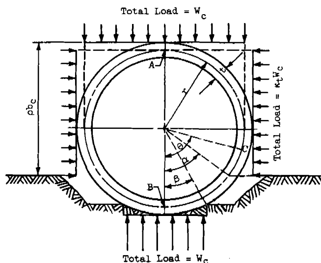
Fig. B-1b Assumed load distribution on an underground conduit installed on a projecting bedding
