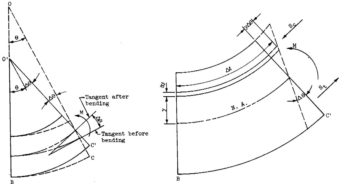
Fig. B-2 Bending of a circular beam caused by a moment at a section
