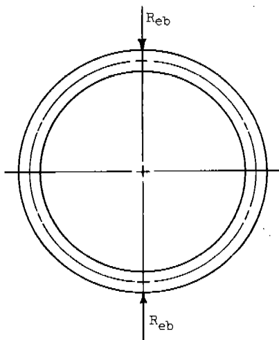
Fig. 2-2a Assumed load distribution for the case of three-edge bearing
