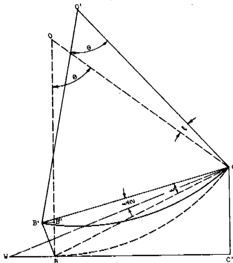
Fig. B-4 Displacement of the end of a circular beam caused by a small rotation at a section
