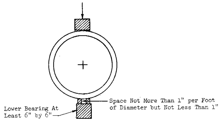
Fig. 2-1 Arrangement of conduit and bearing blocks for standard three-edge bearing laboratory tests of culvert pipe
