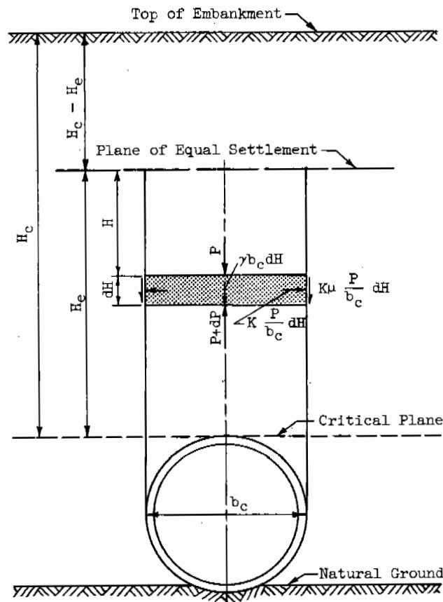
Fig. A-5 Loads on a horizontal element in the interior prism for the incomplete condition
