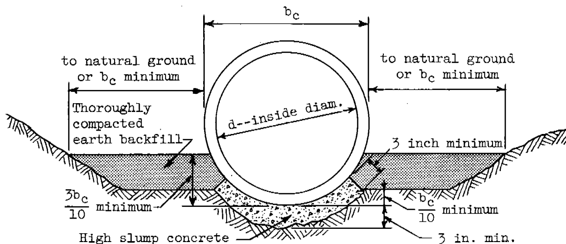
CONSTRUCTION METHOD 1
