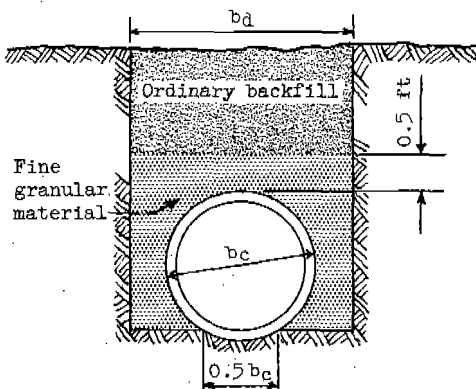
Type C—ordinary bedding
