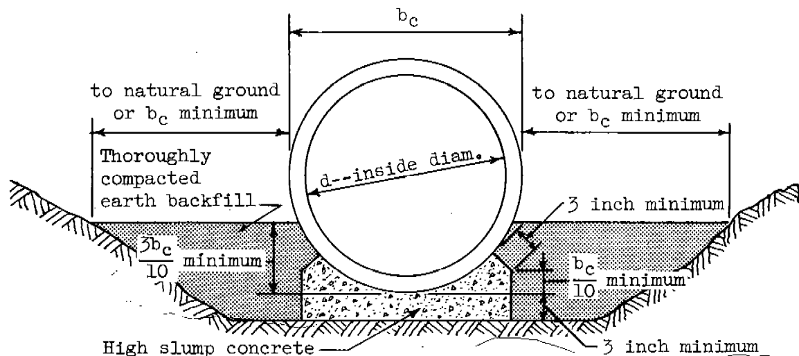
CONSTRUCTION METHOD 2
