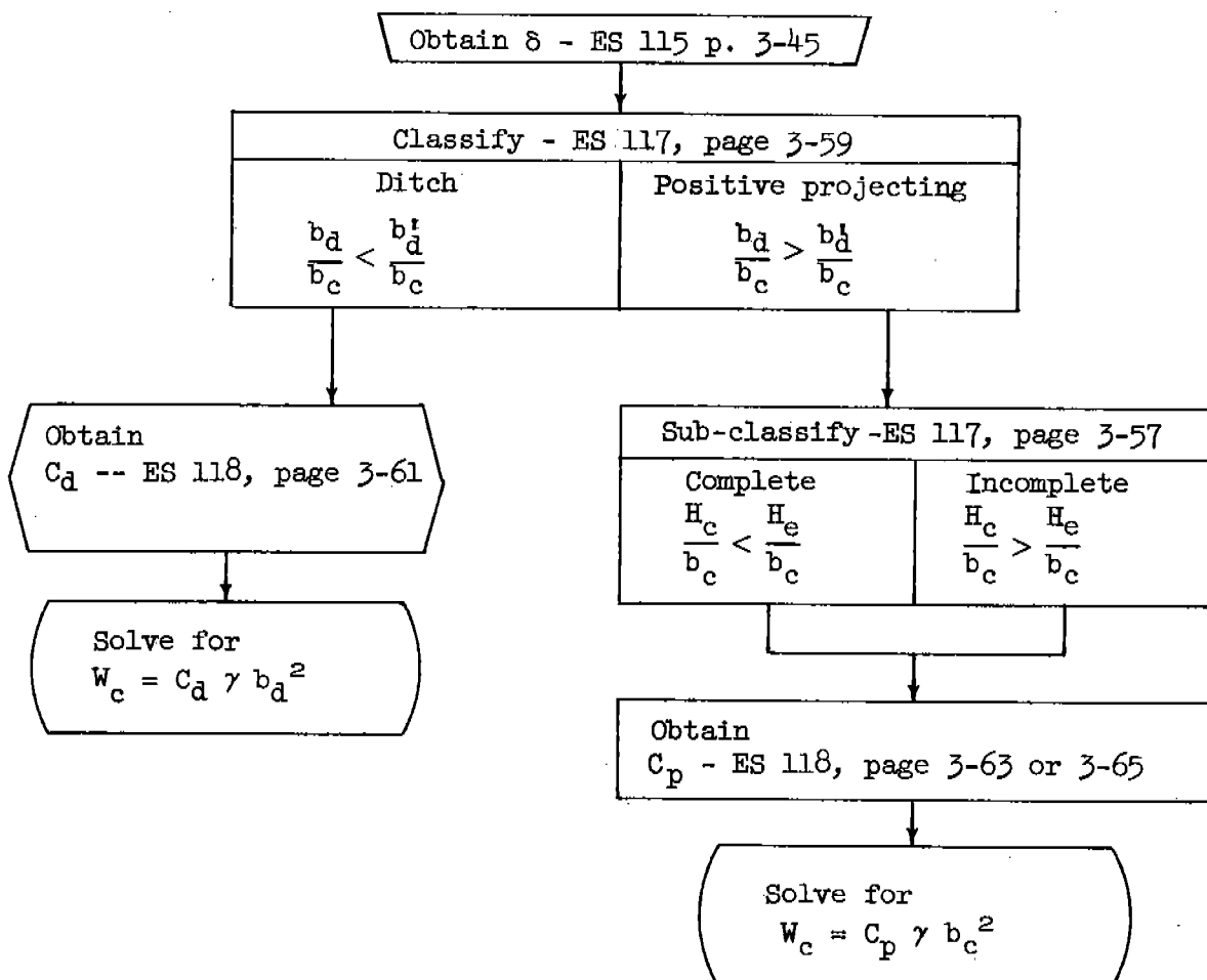
Fig. 1-5. Procedure for determining the load on a ditch conduit or positive projecting conduit.
