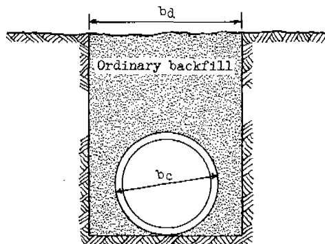
Type D—impermissible bedding
