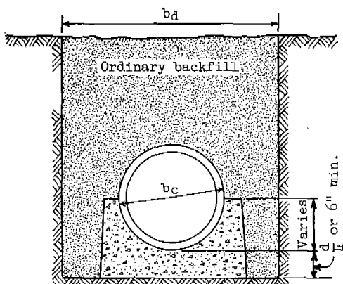
Type A—concrete cradle
