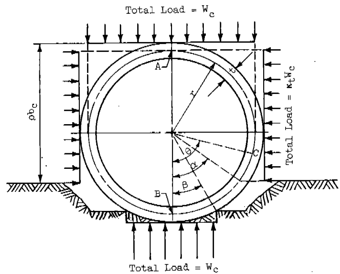
Fig. 2-2b Assumed load distribution on an underground conduit installed on a projecting bedding
