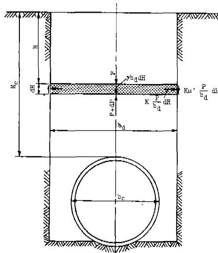
Fig. A-1 Loads on a horizontal element of the backfill material for a ditch conduit
