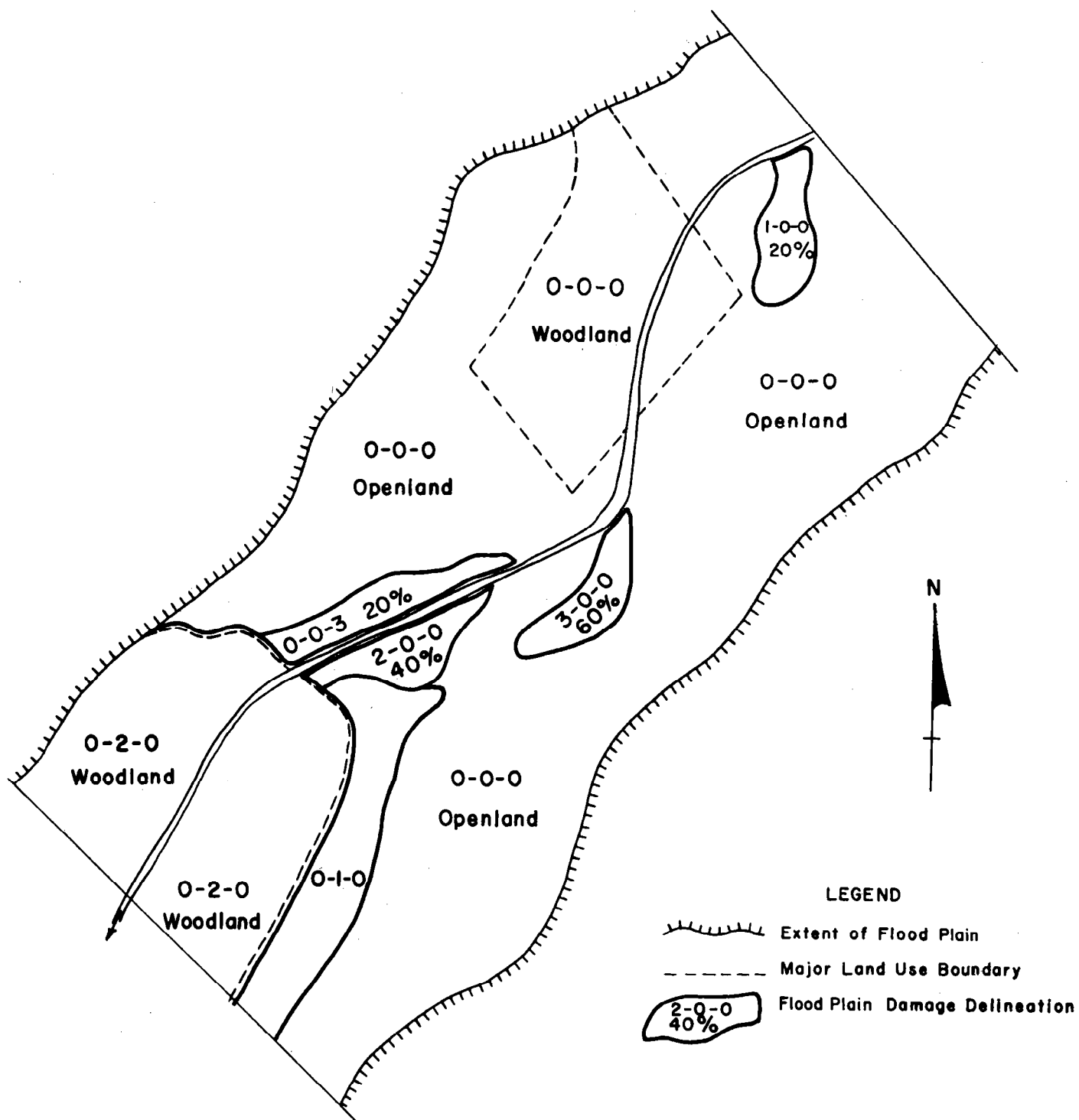
Figure 2-2. Flood Plain Damage Survey - Reach B.
