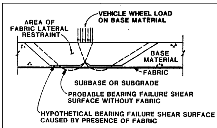
Figure 2 – Shear Failure Mechanism With and Without Geotextile
