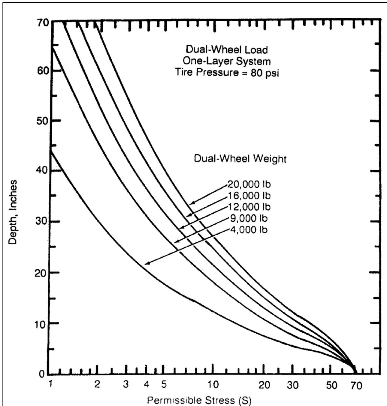
Figure 9 – Dual Wheel Load One-Layer System (Stewart et al., 1977)
