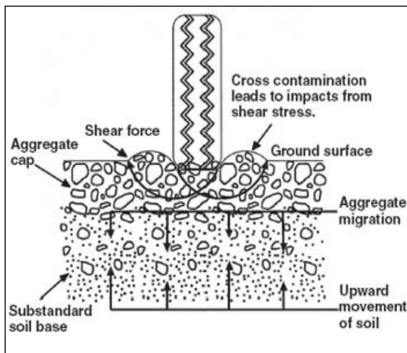
Figure 1 – Failure Mode of Aggregate Surfaced Road (U.S. Forest Service, 2008)
