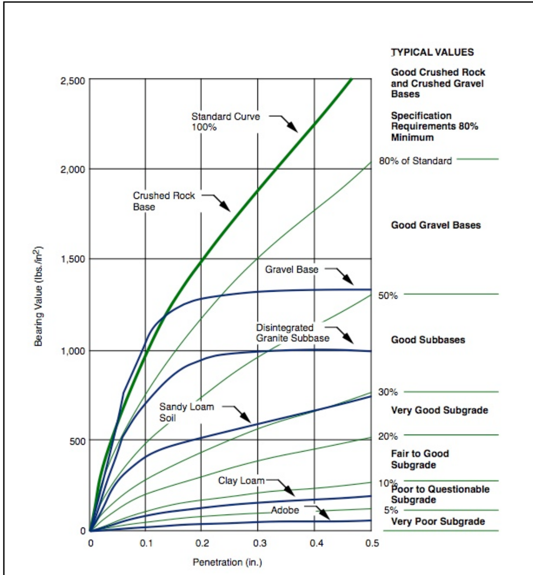
Figure 7 – Typical Bearing Values (psi) Versus Penetration (in.) for Various Materials
