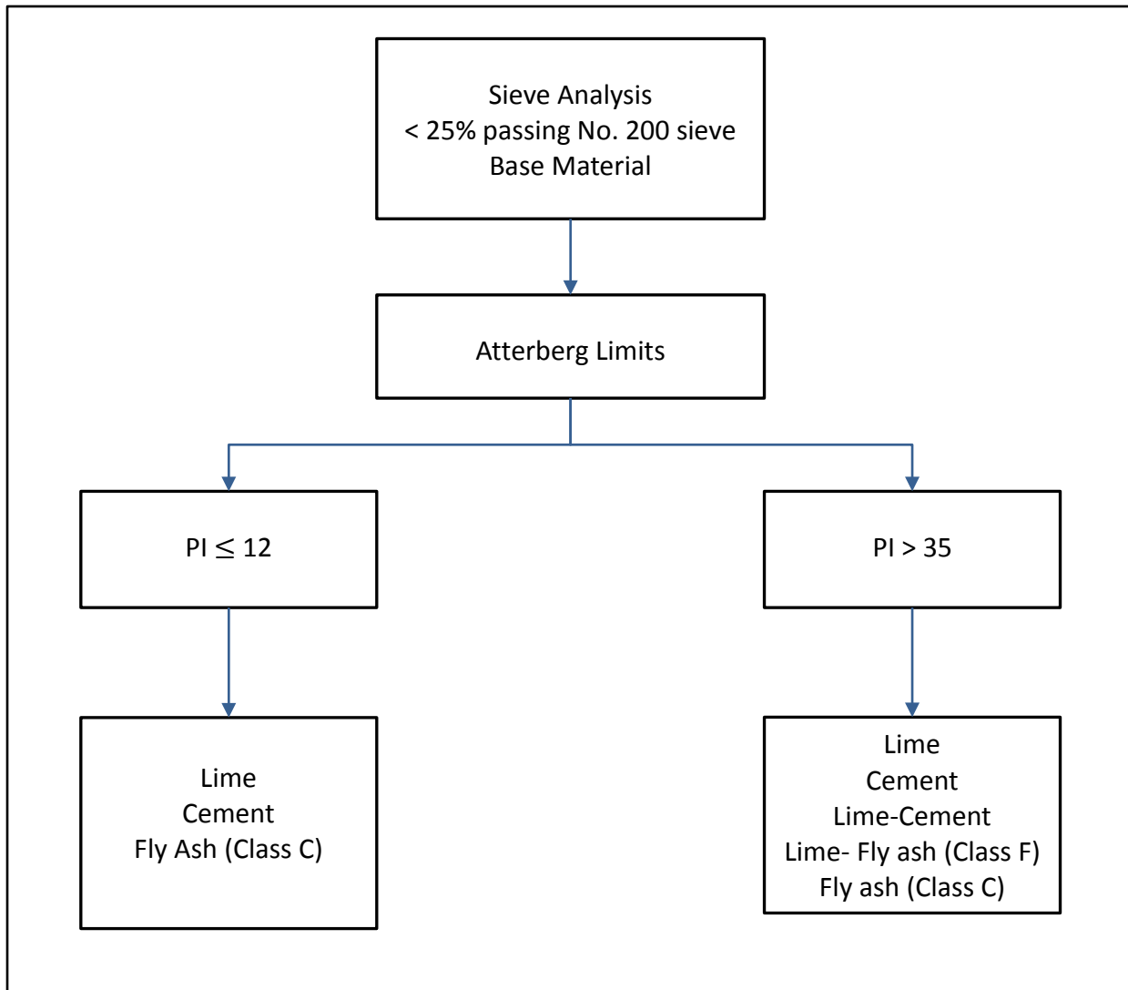
Figure 14 – Decision Tree for Additive Selection for Stabilization of Subgrade
