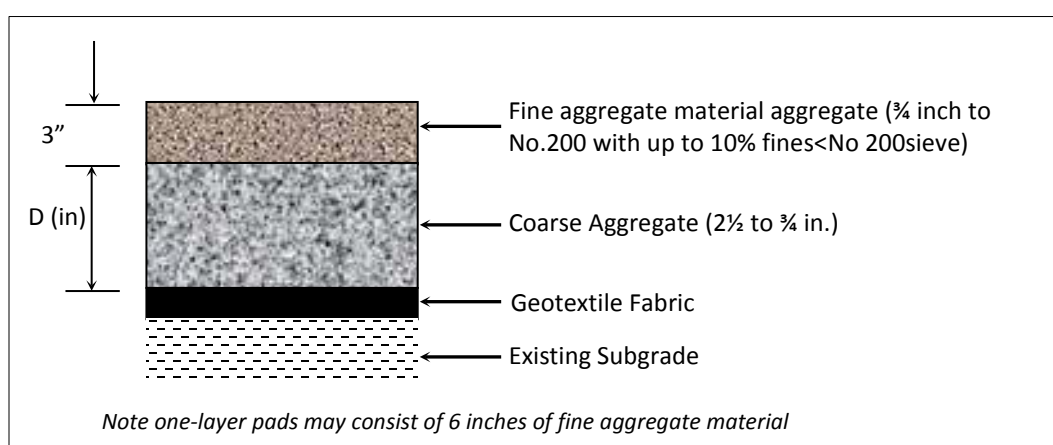
Figure 11 – Details for an Aggregate Pad
