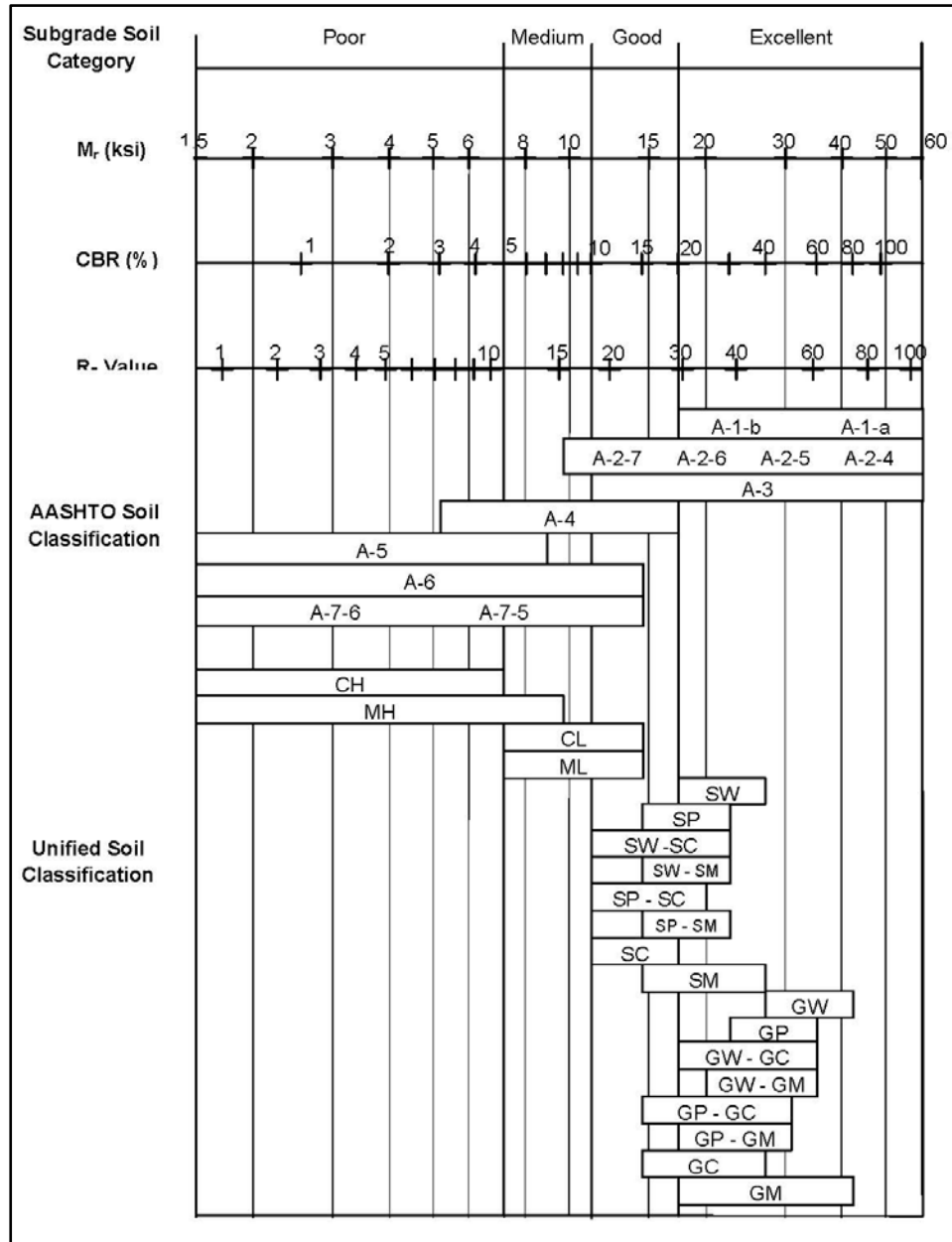
Figure 6 – Correlation of CBR Values With Soil Index (NCHRP, 2001)
