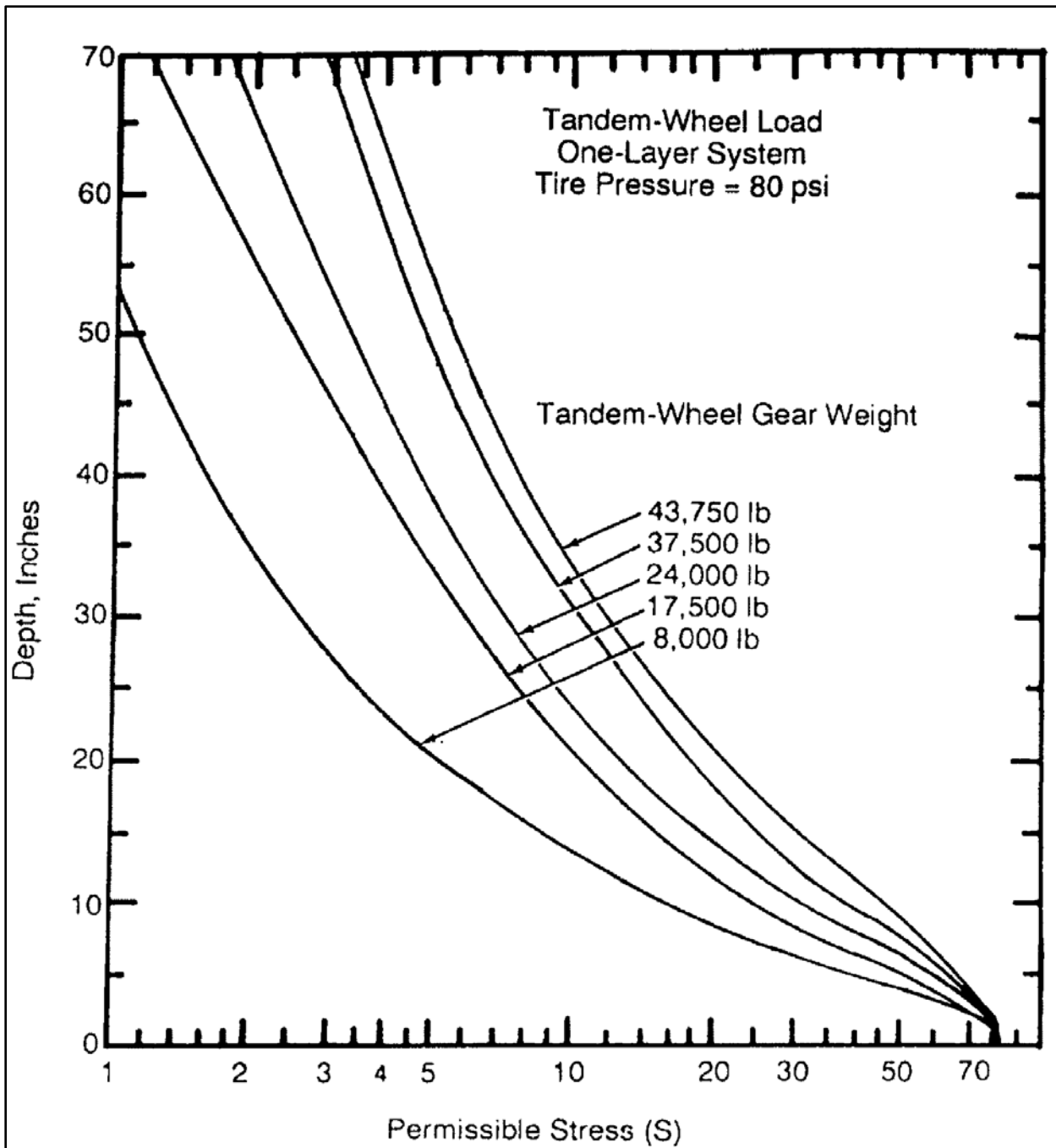
Figure 10 – Tandem Wheel Load One-Layer System (Stewart et al., 1977)
