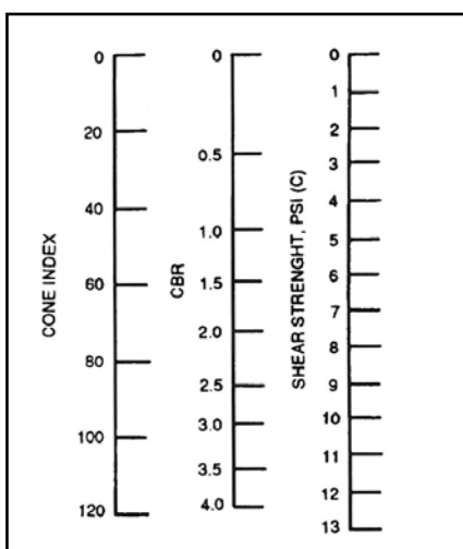
Figure 5 – Relationship Between Shear Strength CBR and Cone Index (U.S. Army, 1995)
