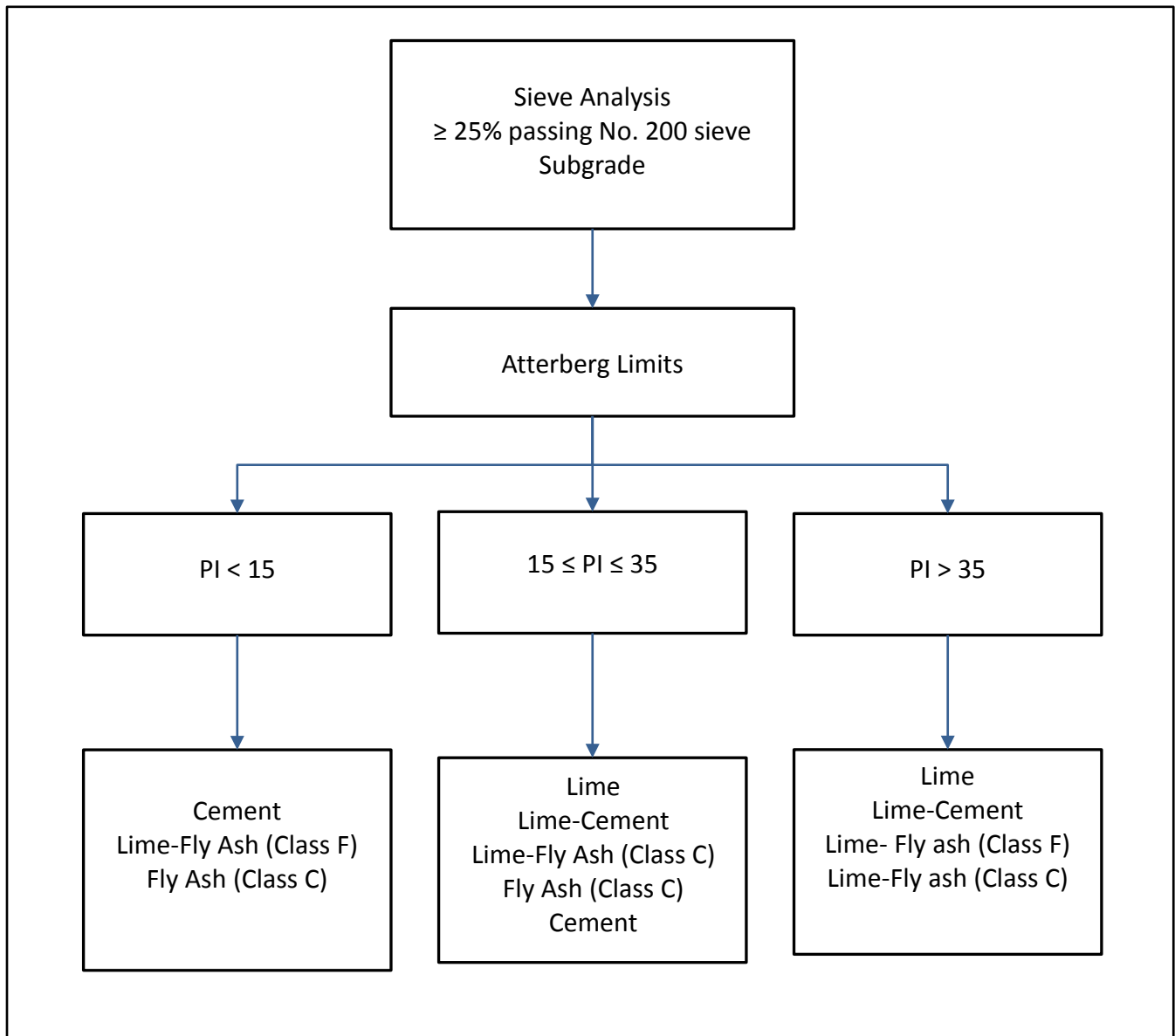
Figure 13 – Decision Tree for Additive Selection for Stabilization of Subgrade
