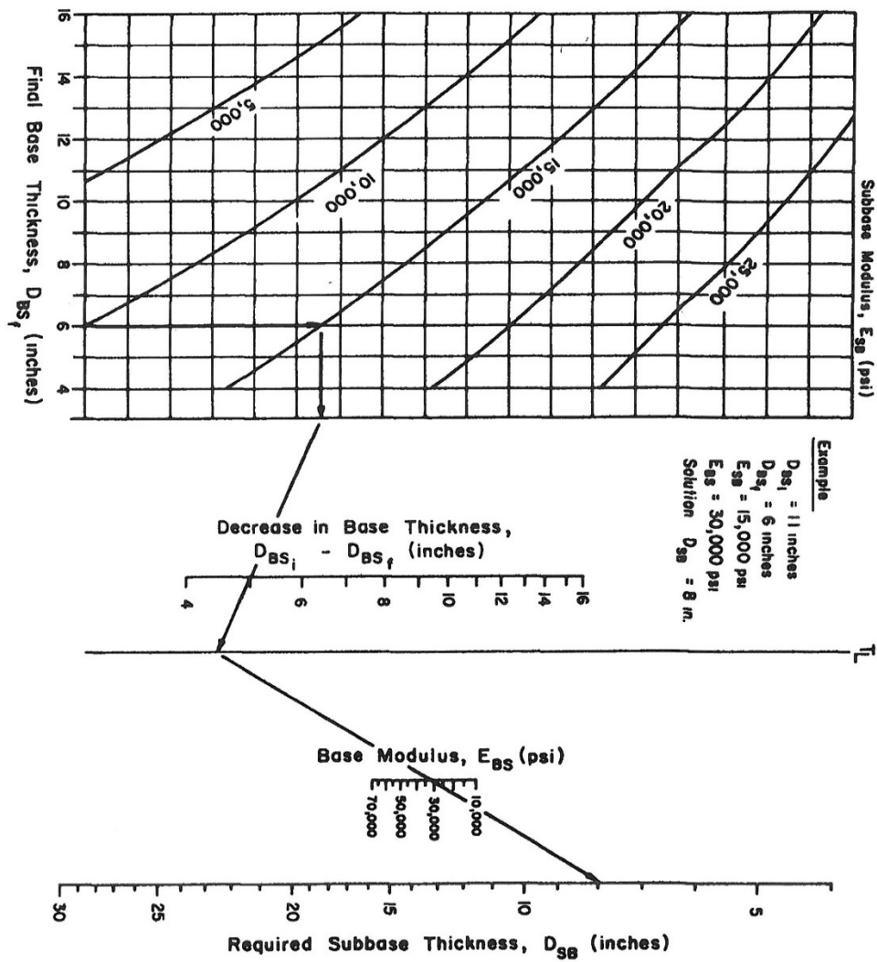
Figure 4.5. Chart to Convert a Portion of the Aggregate Base Layer Thickness To an Equivalent Thickness of Subbase
