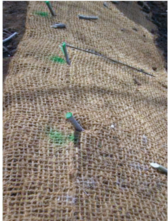
Figure TS14I-39 Live cuttings installed in fabric
