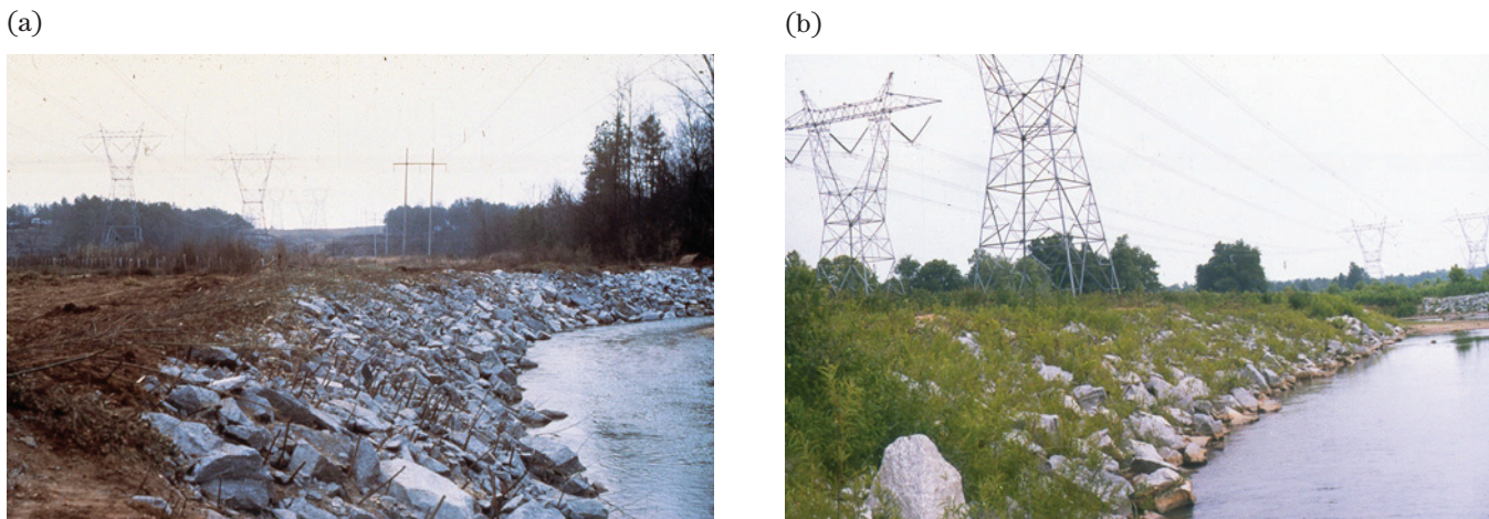
Figure TS14I-25 (a) Completed installation of joint planting; (b) Early in first growing season ( Photo courtesy of Robbin B. Sotir & Associates, Inc. )
