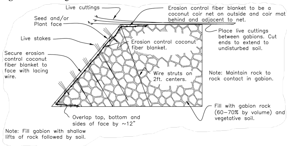
Figure 18-22: Vegetated Gabions
