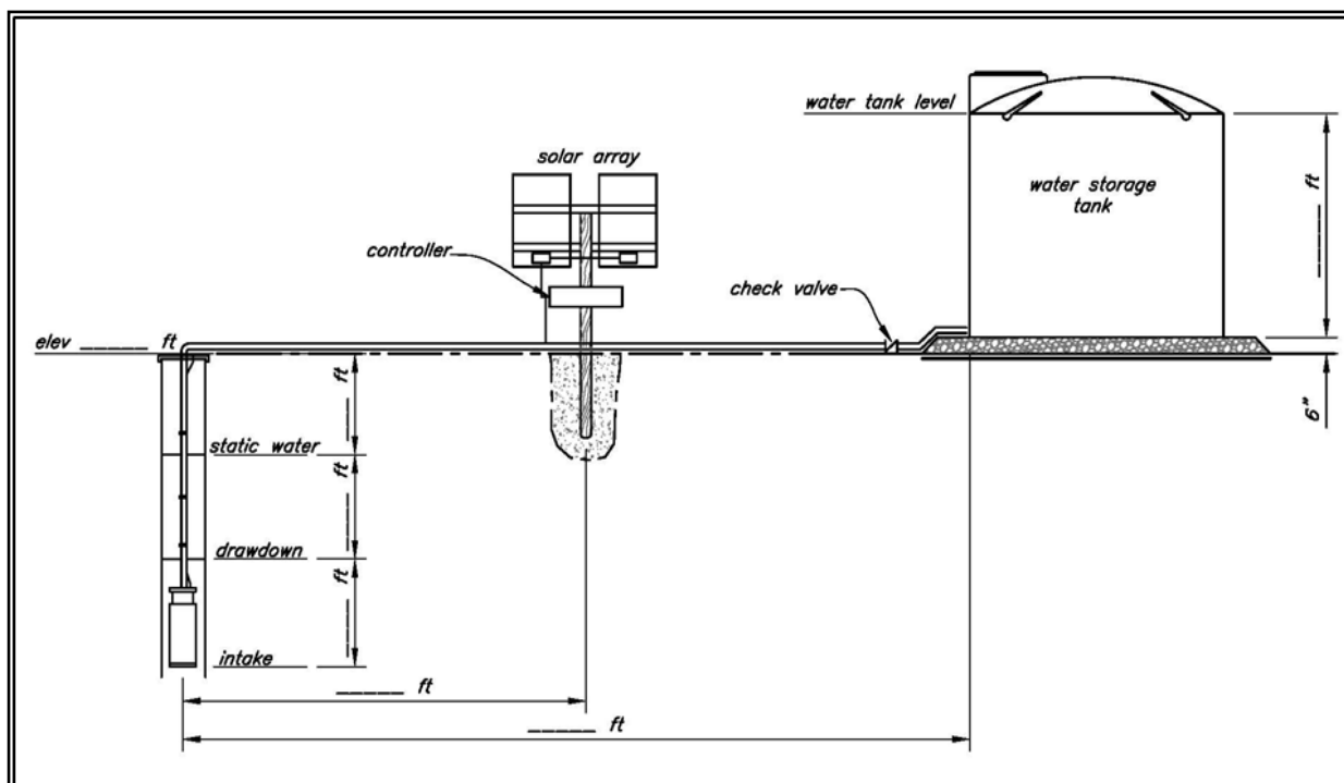
Figure 9 – Typical well installation with pertinent parameters.
