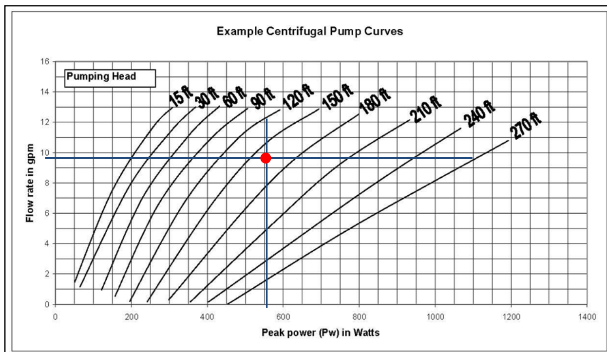
Figure C6 – Pump curves used for Design Example #2.
