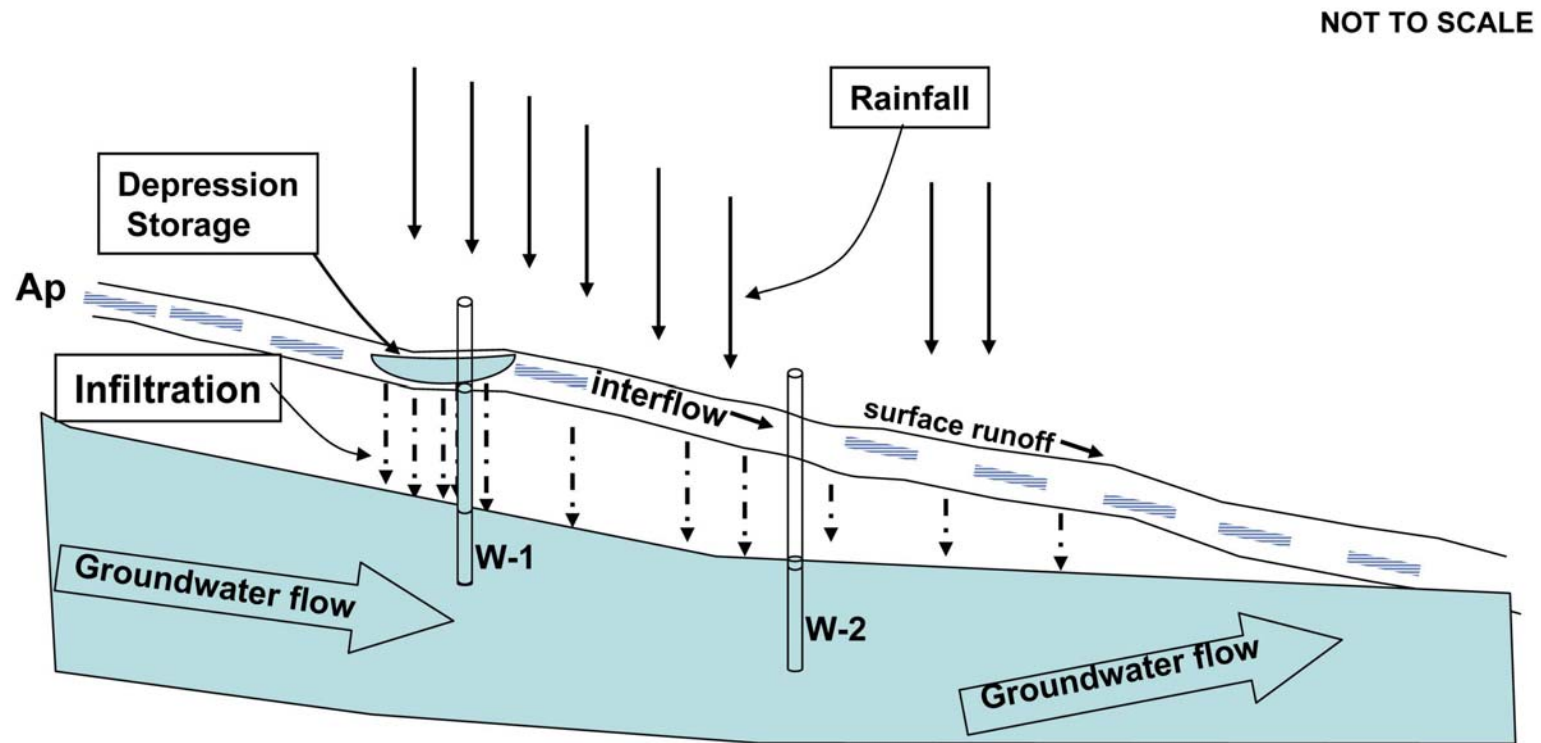
Figure 6. Schematic diagram of paths of water flow significant to shallow water monitoring studies in sloping landscapes. A combination of depression storage and interflow at small scales may be short-lived but can be significant enough to cause bypass flow down poorly protected well risers (W-1). Figure modified from Kirkby (1969).
