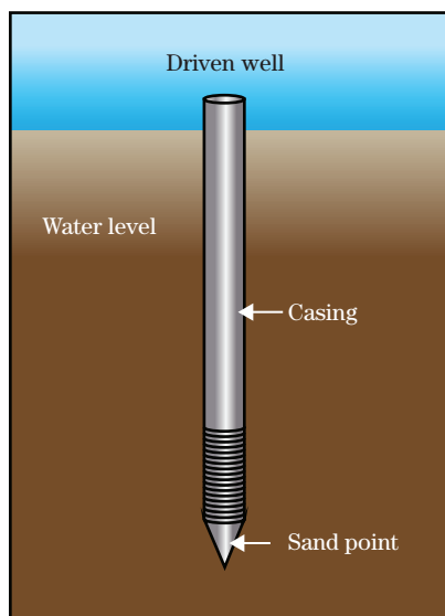
Figure 12–17 Sand point used for small diameter driven well
