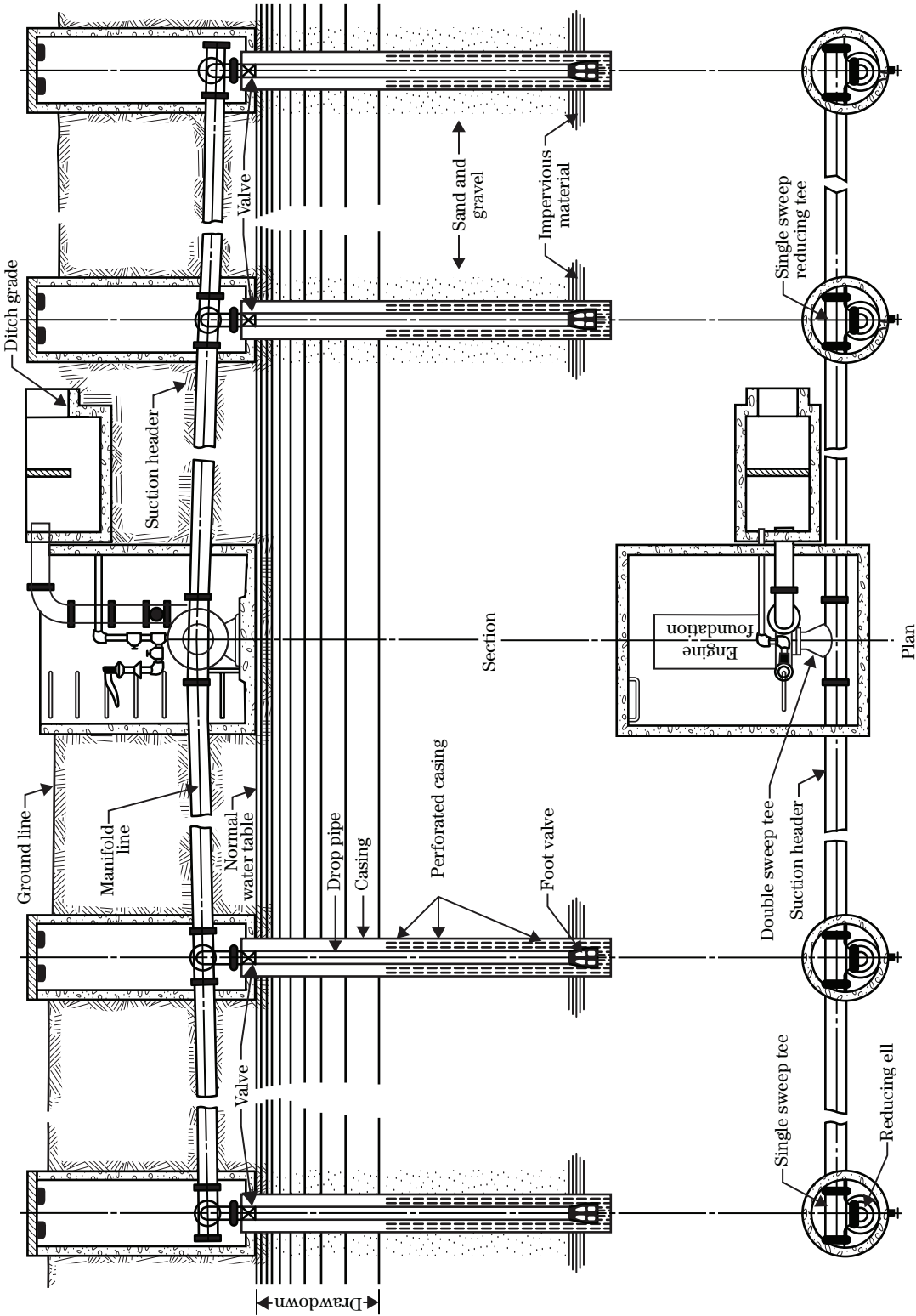
Figure 12-25 Typical manifold multiple-well system. Note that the pump may be an engine or electric motor
