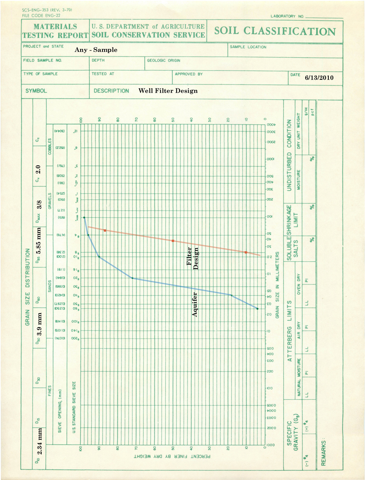
Figure 12-23 Filter design gradation, based on aquifer particle size distribution
