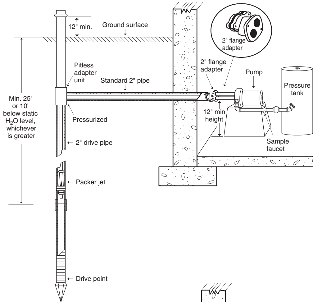
Figure 3. Deep-well offset pump installation using a packer-jet assembly in a 2 inch diameter well.
