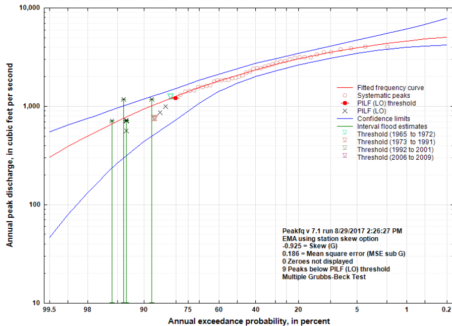
Figure 10.11. Graph showing annual exceedance probability plot for USGS gage 05489490 Bear Creek at Ottumwa, Iowa based on flood frequency analysis using Expected Moments Algorithm with Multiple Grubbs-Beck Test. The red line is the fitted log-Pearson Type III frequency curve, the blue lines are the upper and lower confidence limits, the red circles are the systematic peaks, the green lines represent the interval flood estimates, the solid red circle with a line through it is the potentially influential low floods (PILFs) thresholds as identified by the MGBT, and the black x's are the PILFs identified by the MGBT.
